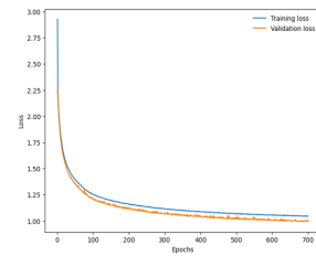
Figure 3: Training loss and validation loss for learning rate 0.0007
