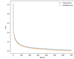
Figure 2: Training loss and validation loss for learning rate 0.0005
