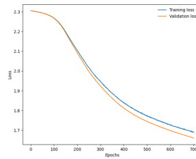
Figure 1: Training loss and validation loss for learning rate 0.00001
