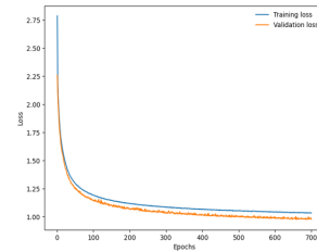
Figure 4: Training loss and validation loss for learning rate 0.001
